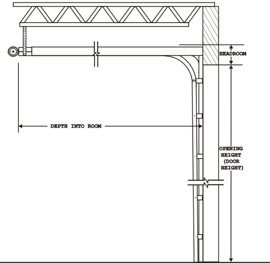
SIDE VIEW OF TRACK
