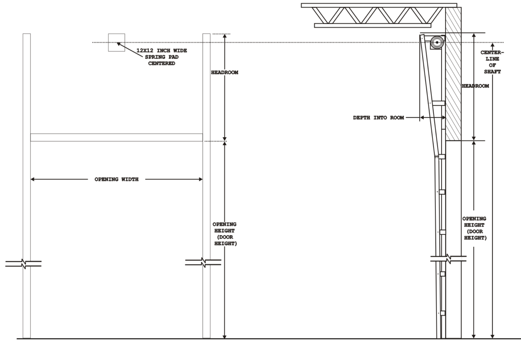
INTERIOR ELEVATION
