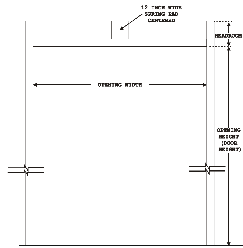
INTERIOR ELEVATION
